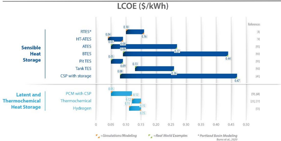
Figure 3: Estimate levelized Cost of Energy for RTES and other selected Thermal Energy Storage Systems. Aquifer Thermal Energy Storage (ATES); High-Temperature (HT) ATES; Borehole Thermal Energy Storage (BTES); Concentrated Solar Power (CSP); Phase Change Material (PCM). Source: See footnote 13.
