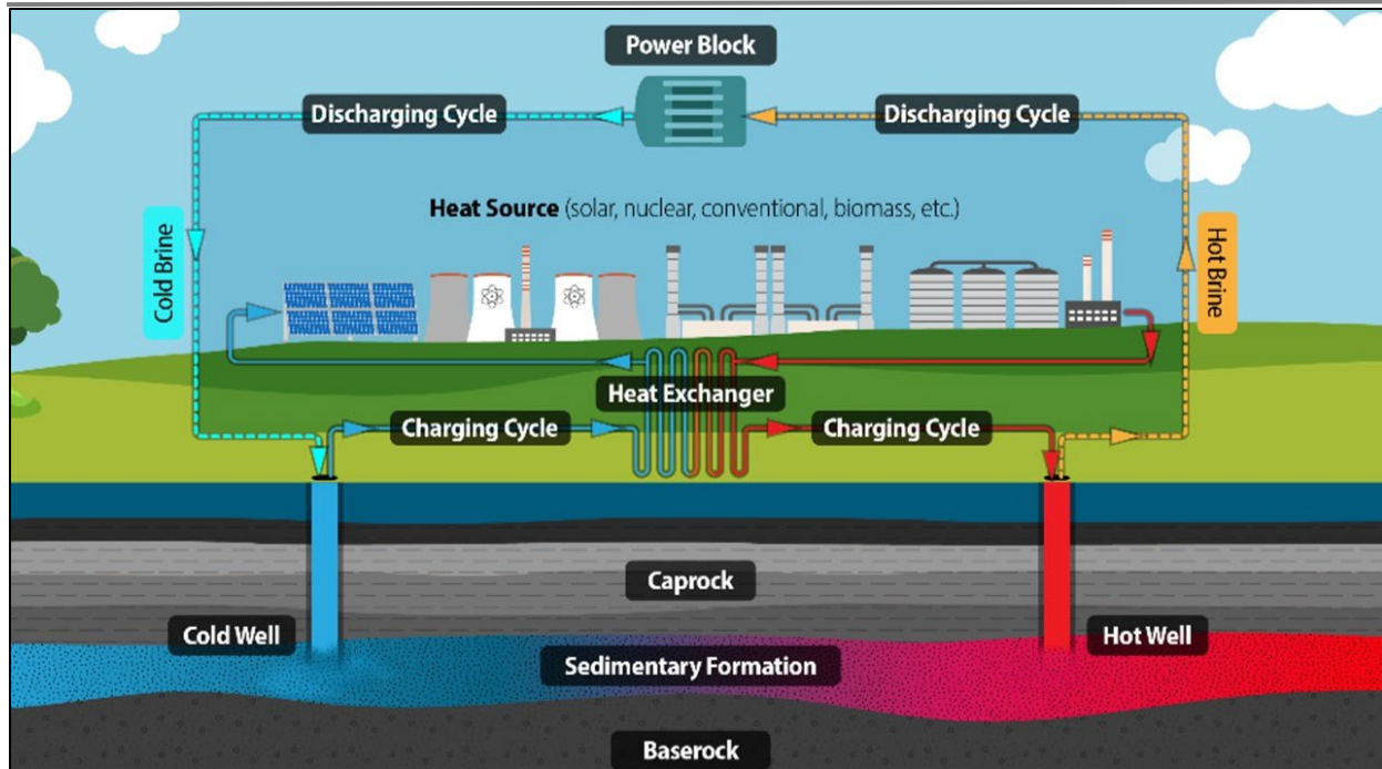
Figure 2: Schematic Diagram of a Notional RTES System.
