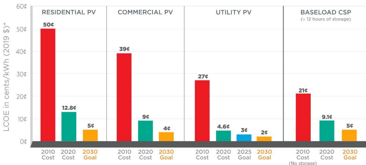
Figure 1. Solar energy cost reductions 2010-2020 and DOE cost goals without federal tax credits or state/local incentives.
