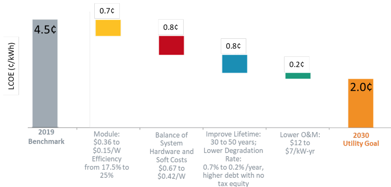
Figure 2. One pathway to SETO's 2030 utility-scale PV cost goal.
